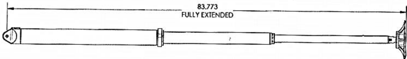
JACK COMPRESSED AND EXTENDED DIMENSIONS
