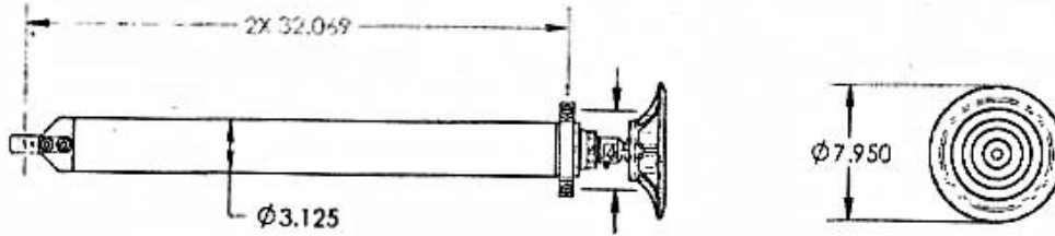
JACK MOUNTING POINT LOCATIONS
